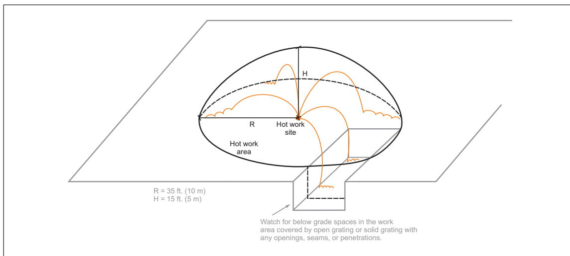
Fig. 2. Hot work permit-required area with single hot work site
