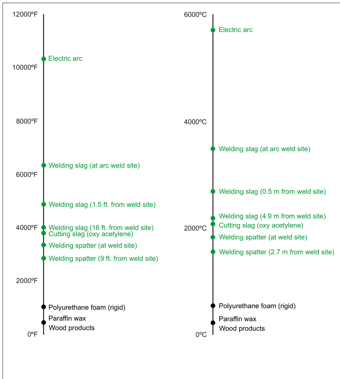
Fig. 6. Hot work ignition source temperature vs. solid-fuel ignition temperature
