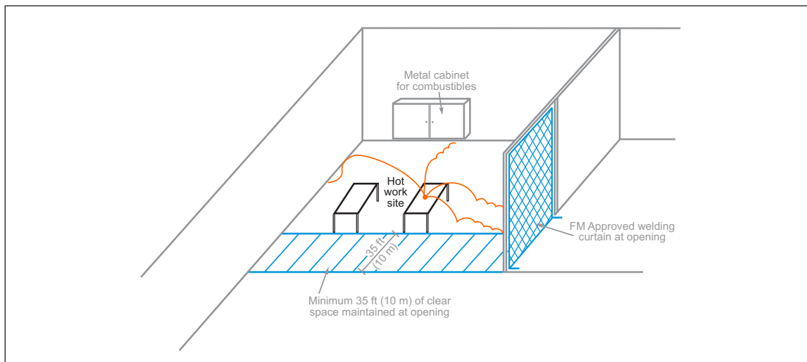
Fig. 1. Hot work designated area
