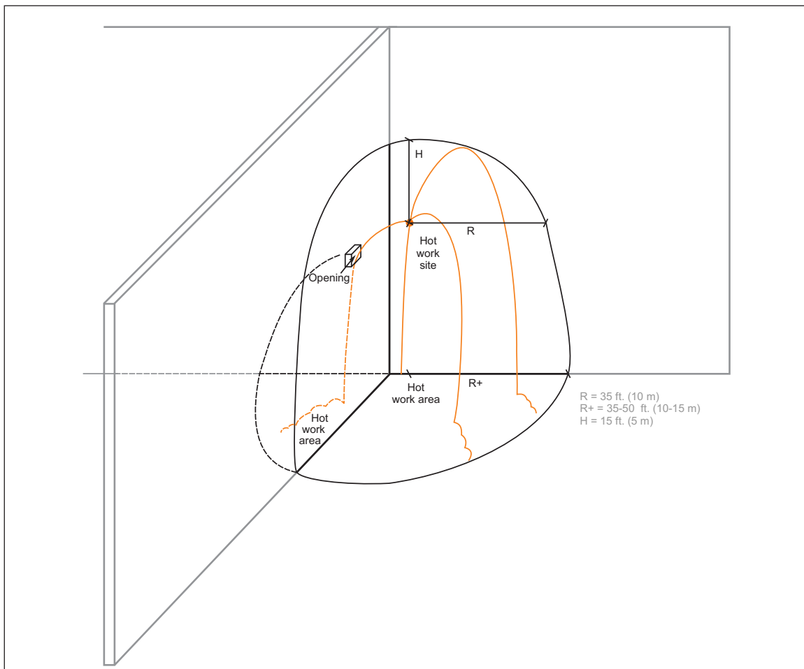
Fig. 5. Elevated hot work permit-required area
