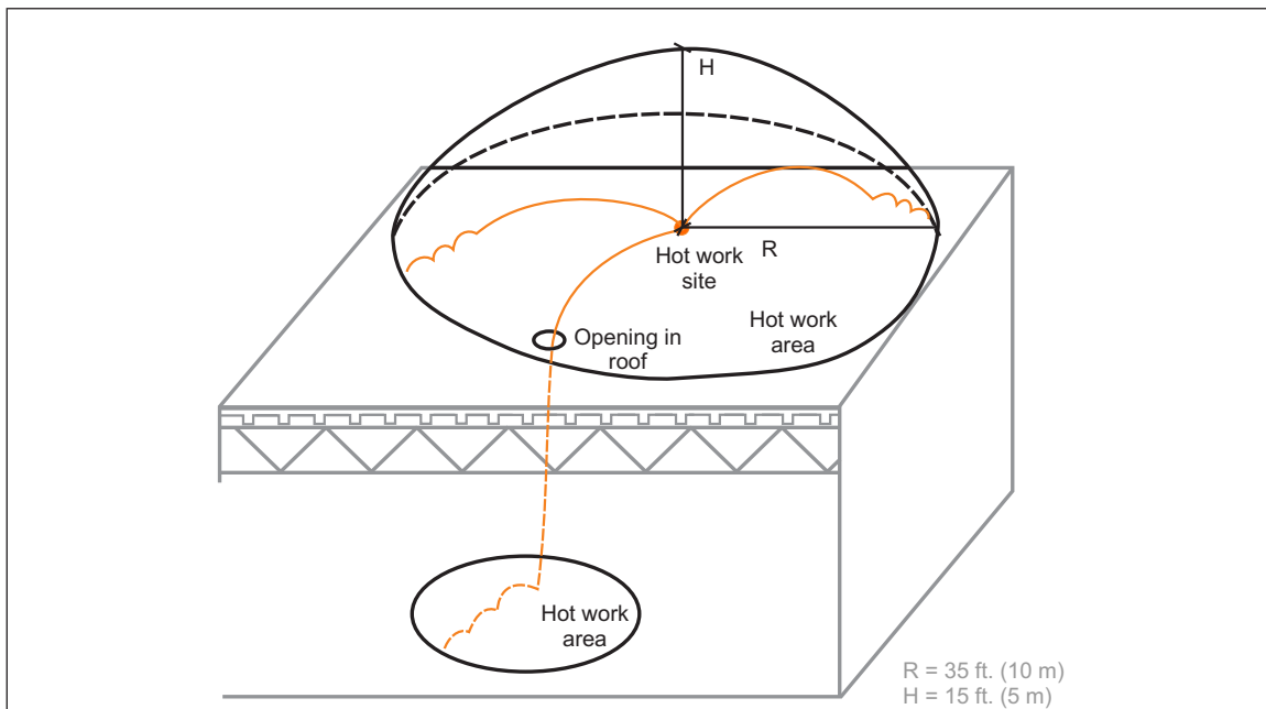
Fig. 4. Rooftop hot work permit-required area
