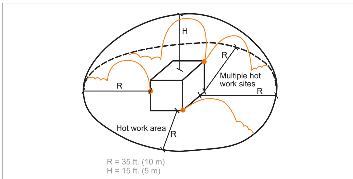
Fig. 3. Hot work permit-required area with multiple hot work sites
